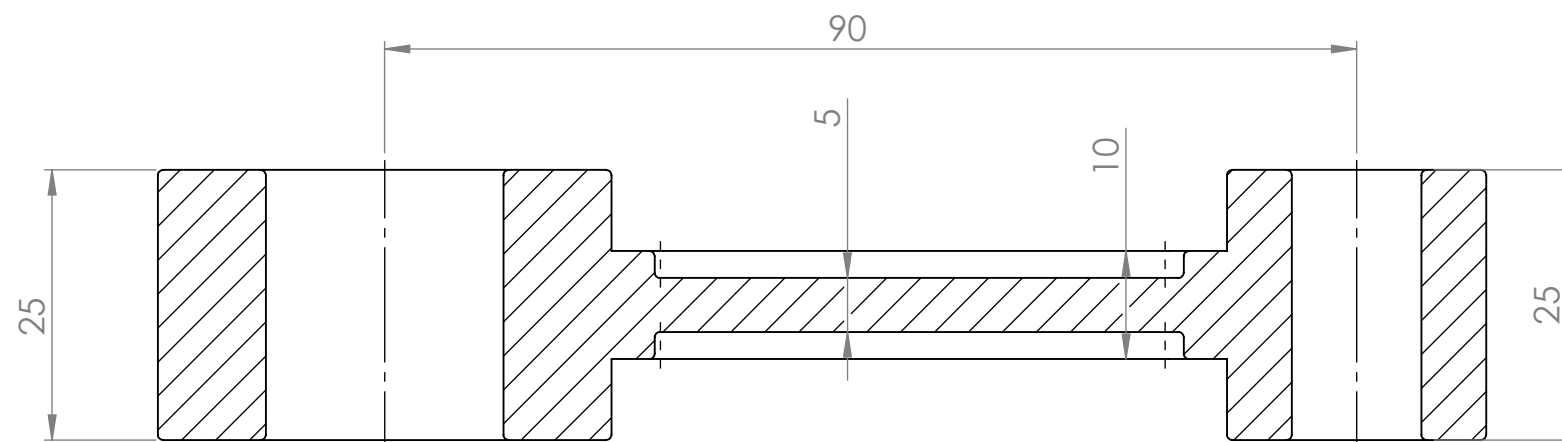
SECTION B-B
